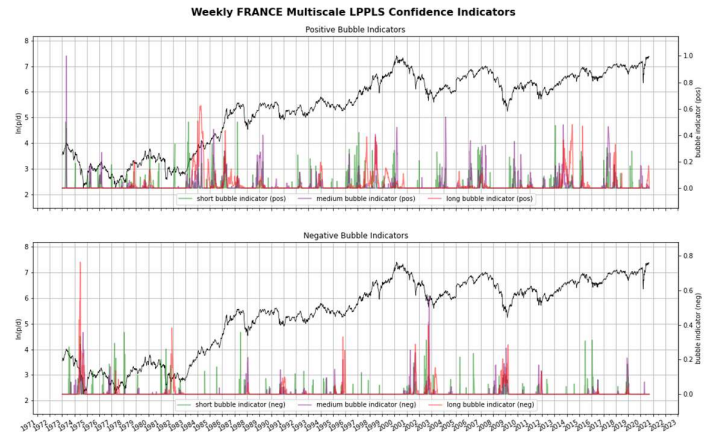
Figure 2: Multi-Scale Log-Periodic Power Law Singularity Confidence Indicators (MS-LPPLS-CIs) of the G7 Countries.
