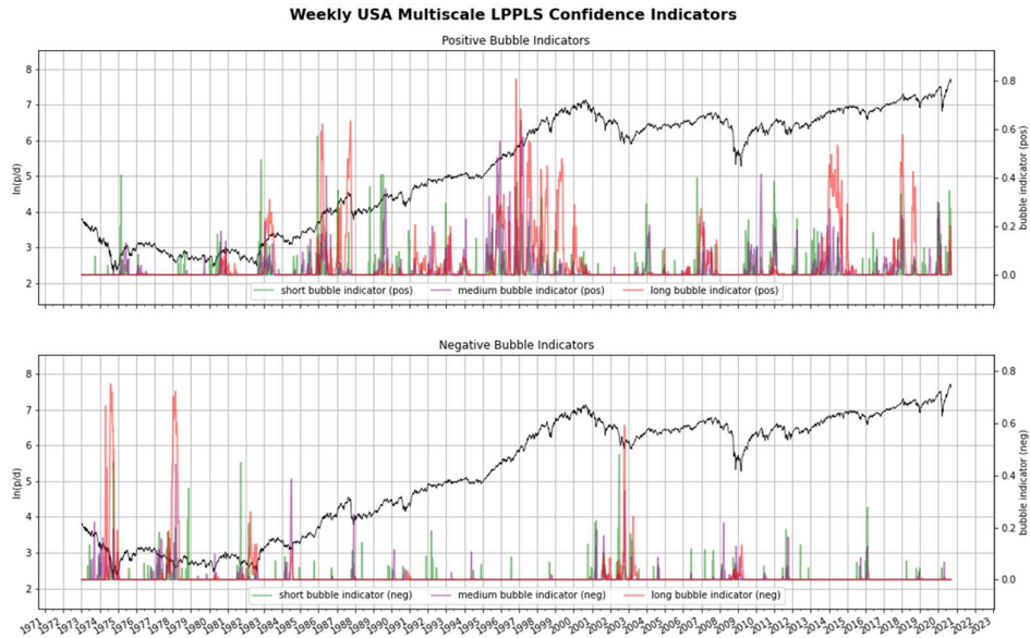
Figure 1 (a): Multi-Scale Log-Periodic Power Law Singularity Confidence Indicators (MS-LPPLS-CIs)
