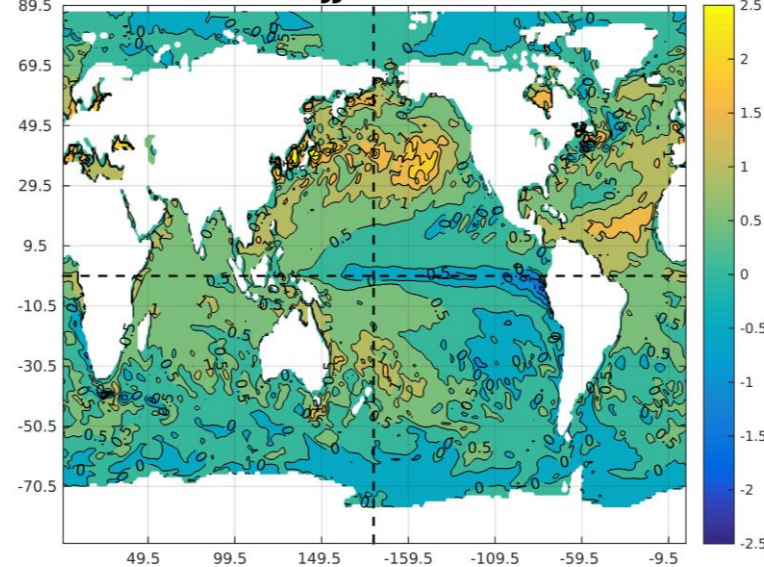
SST MJJ IC:Mar2024
