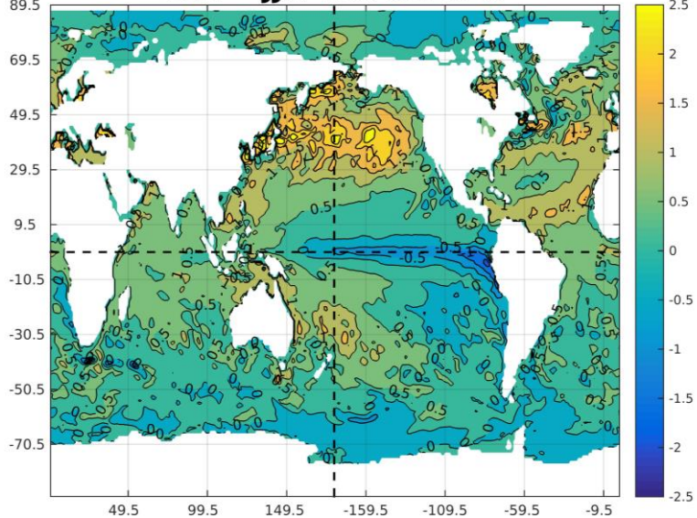
SST JJA IC:Mar2024
