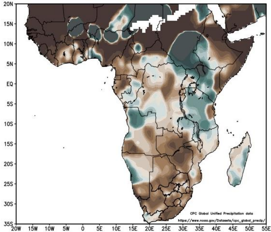
Rainfall (% of normal): February 2024 February long-term mean: 1981–2010
