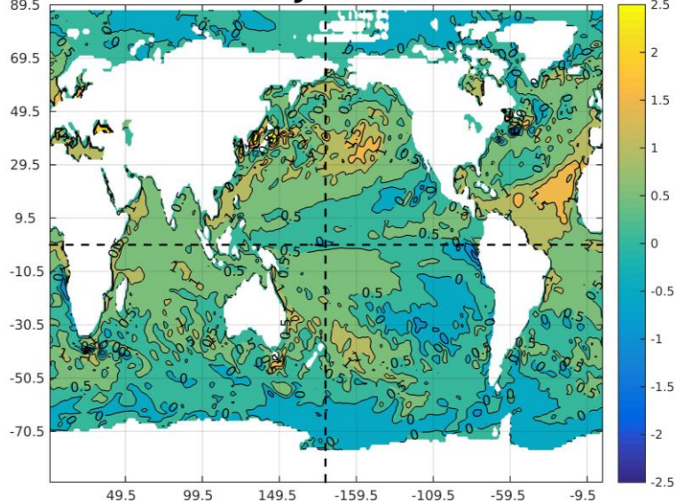
SST AMJ IC:Mar2024
