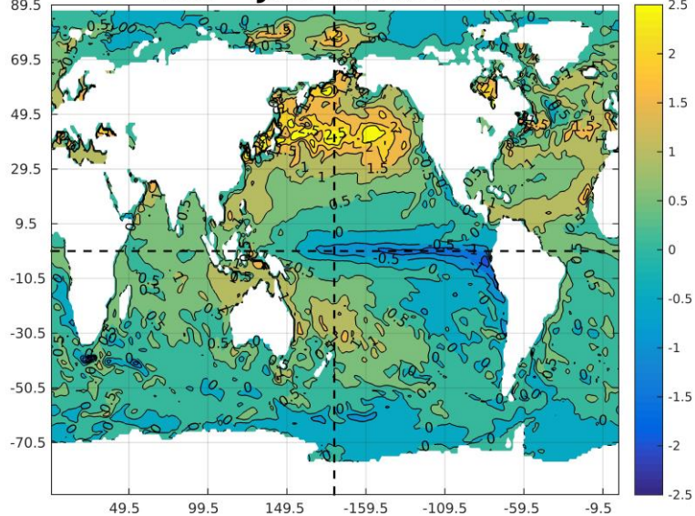
SST JAS IC:Mar2024
