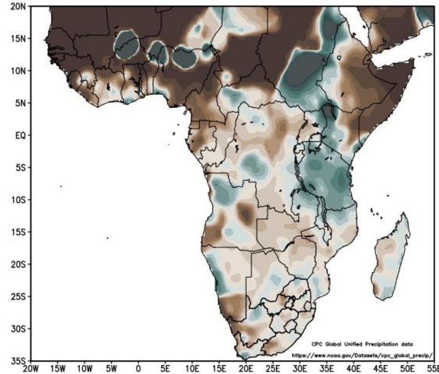
Rainfall (% of normal): December–January–February 2023/24 December–January–February long-term mean: 1981/82–2010/11
