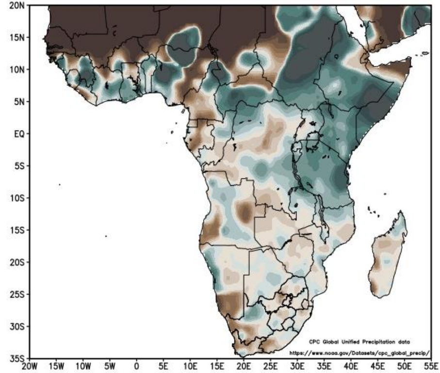
Rainfall (% of normal): November–December–January 2023/24 November–December–January long-term mean: 1981/82–2010/11
