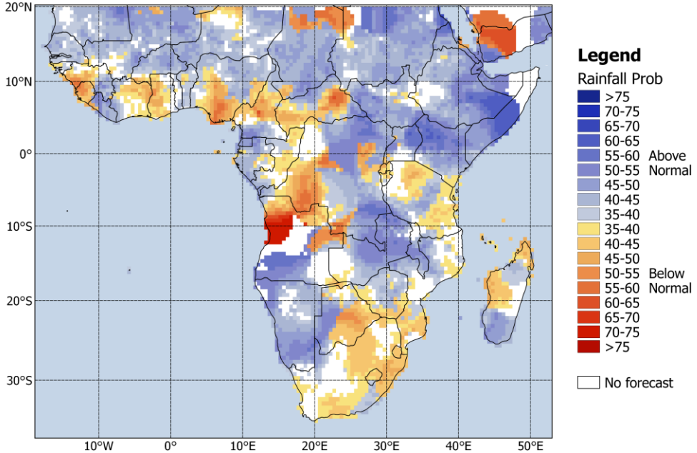
MJJ 2025 Rainfall; ICs: Apr
