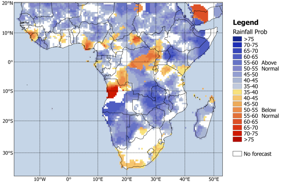
MJJ 2025 Rainfall; ICs: Feb
