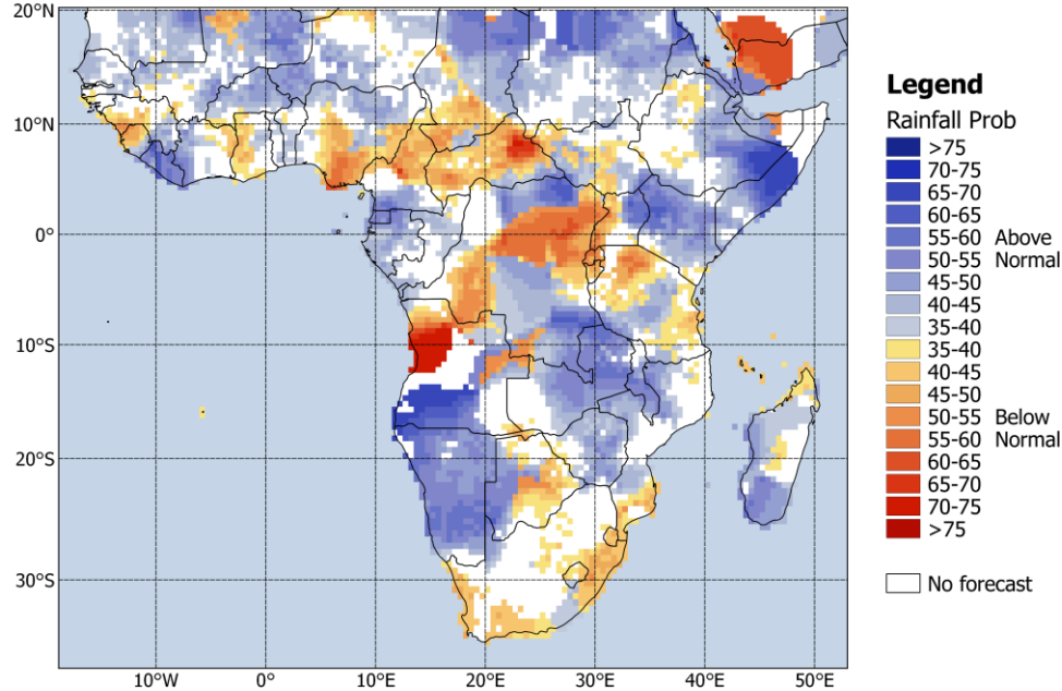
MJJ 2025 Rainfall; ICs: May
