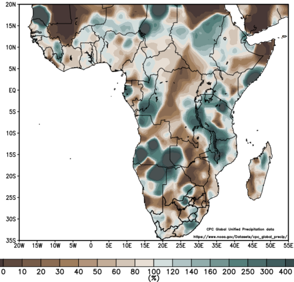
Rainfall (% of normal): May–June–July 2025 May–June–July long-term mean: 1981–2010
