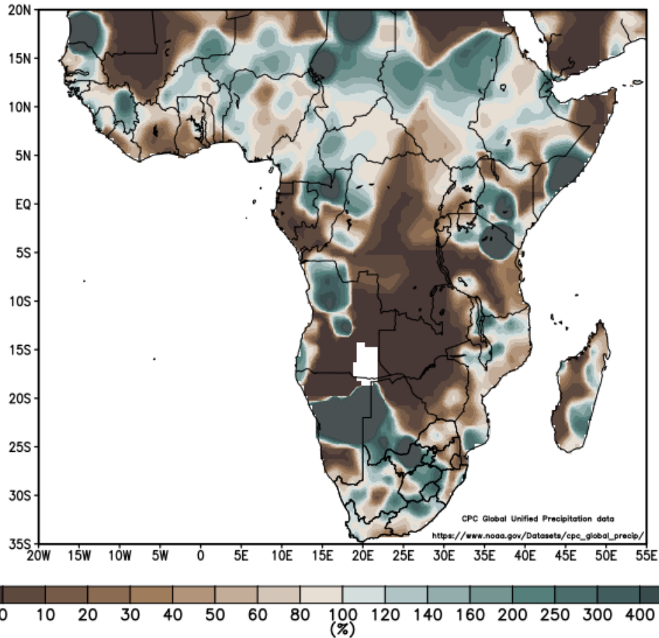
Rainfall (% of normal): July 2025 July long-term mean: 1981–2010
