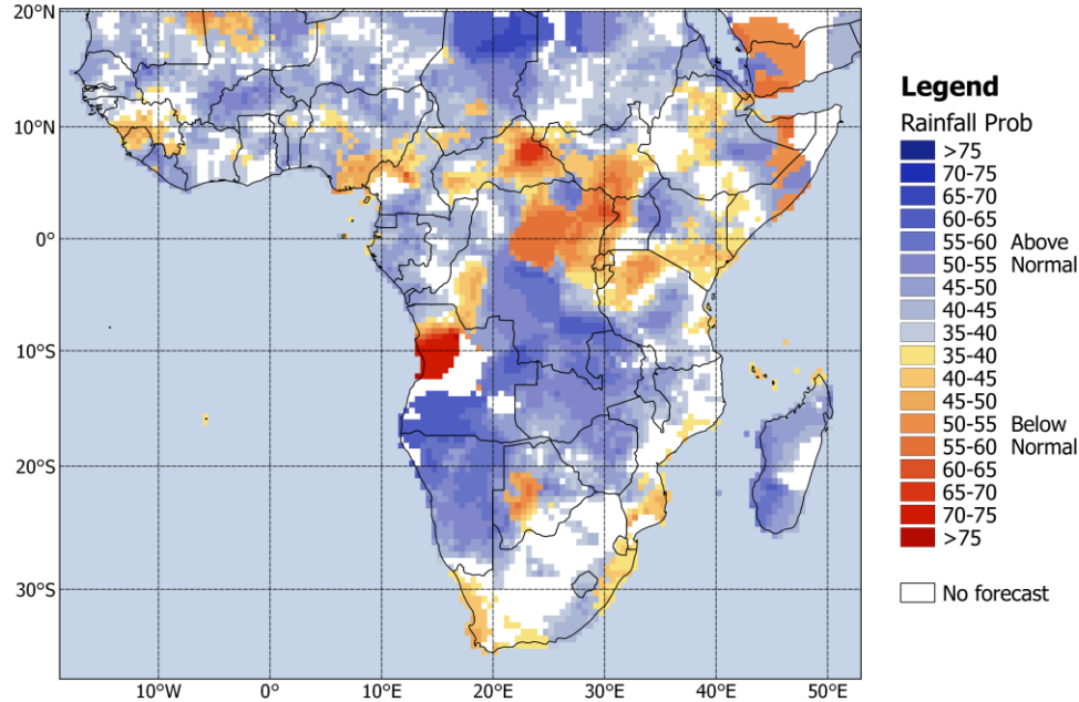
MJJ 2025 Rainfall; ICs: Mar
