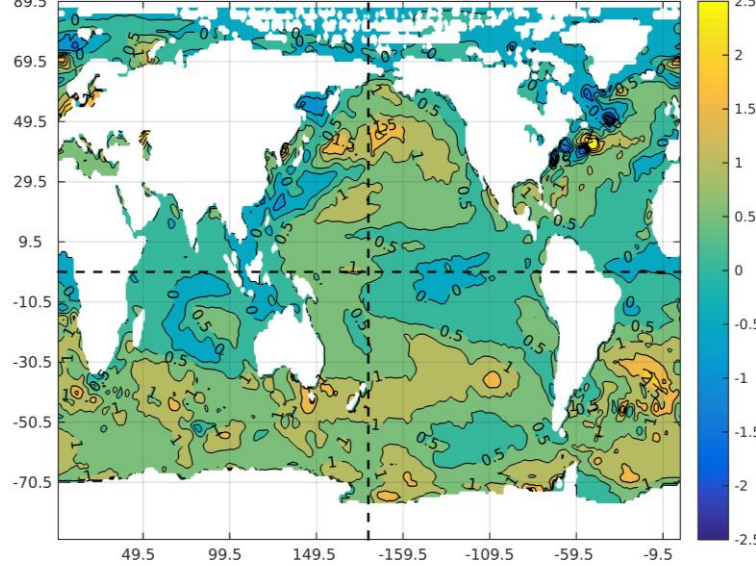
SST JFM IC:Aug2025
