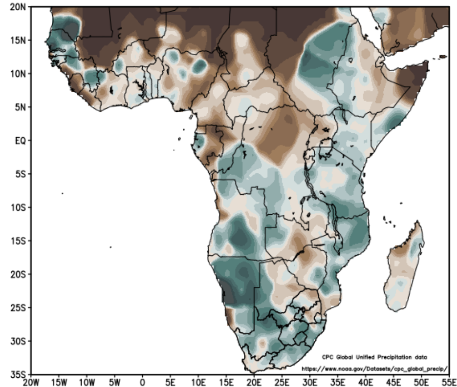
Rainfall (% of normal): March–April–May 2025 March–April–May long-term mean: 1981–2010
