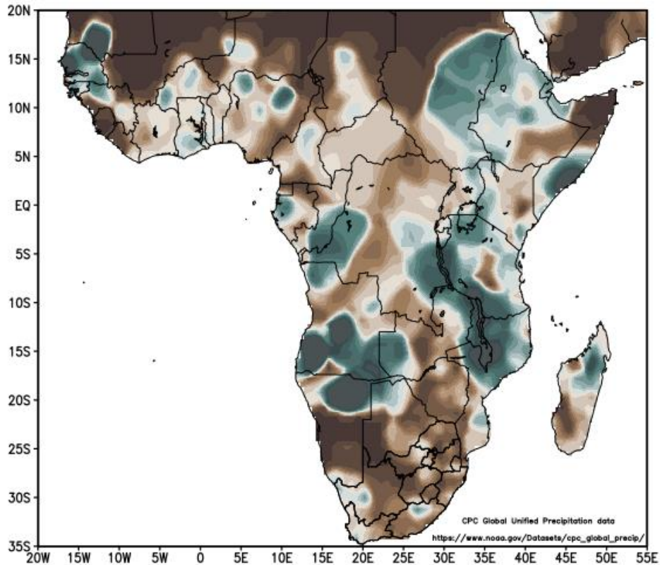
Rainfall (% of normal): May 2025 May long-term mean: 1981–2010
