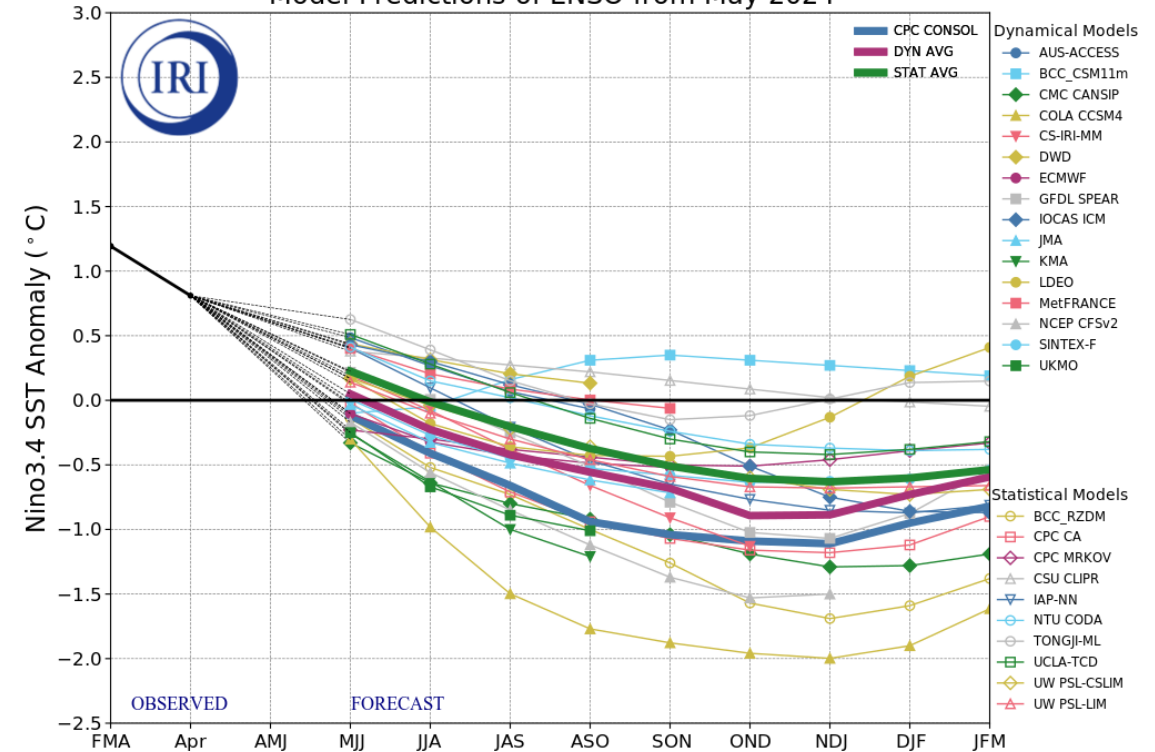
Model Predictions of ENSO from May 2024
