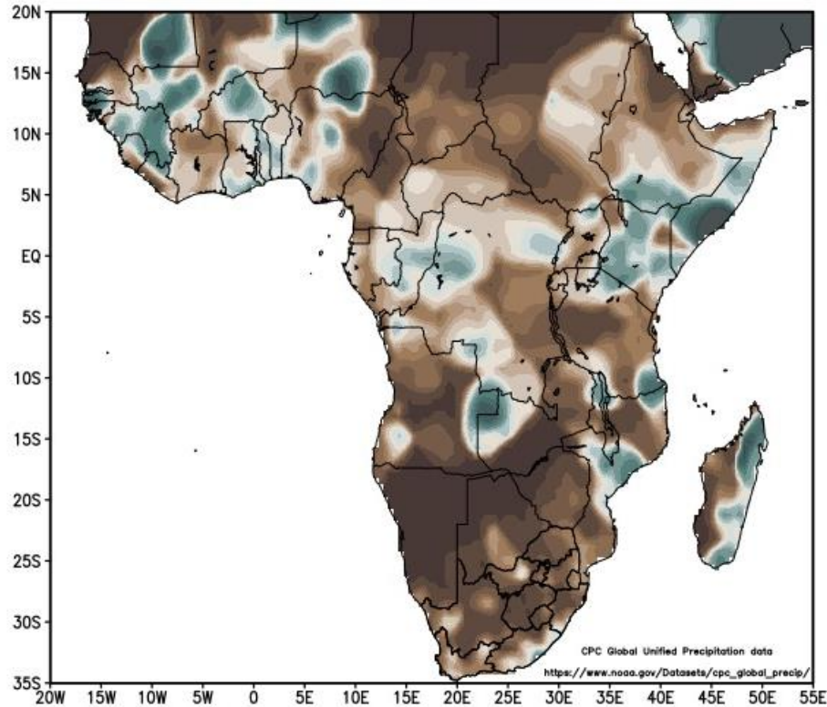
Rainfall (% of normal): May 2024 May long-term mean: 1981–2010
