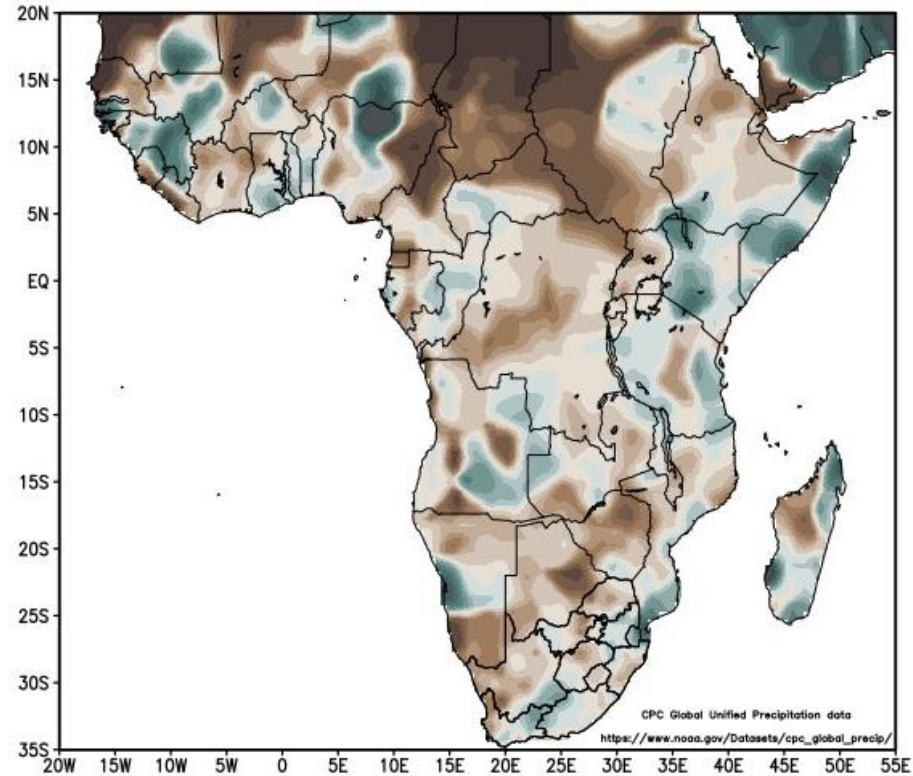
Rainfall (% of normal): March–April–May 2024 March–April–May long-term mean: 1981–2010
