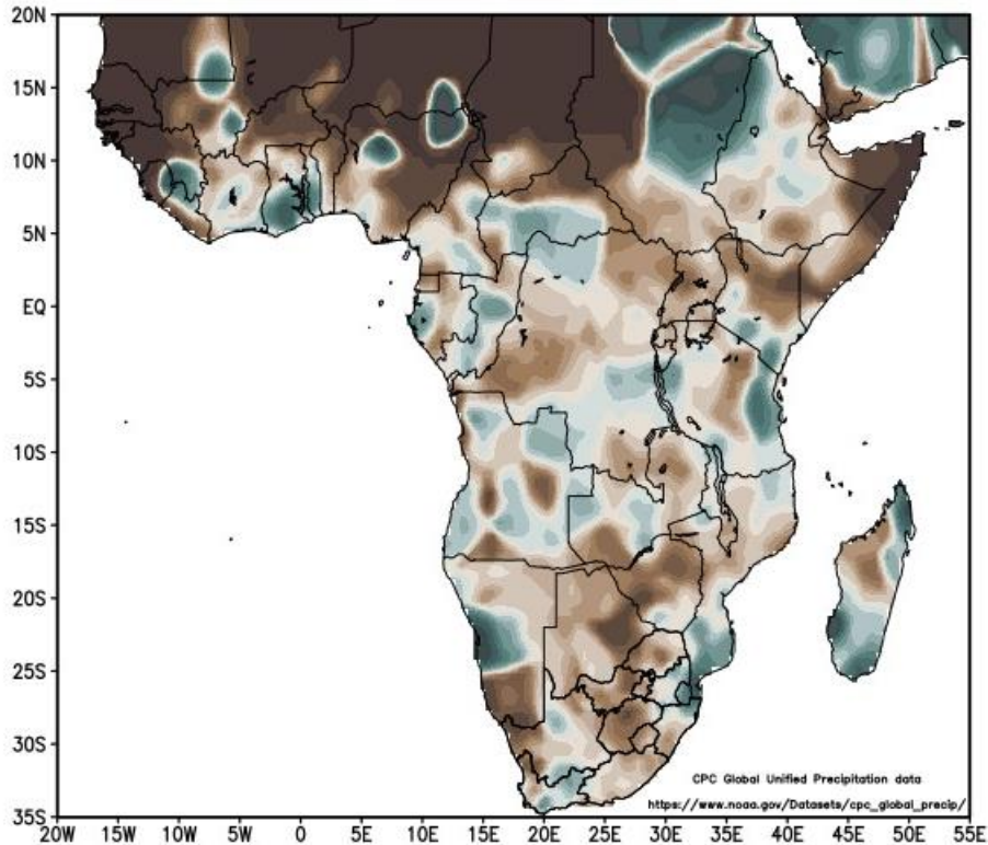
Rainfall (% of normal): March 2024 March long-term mean: 1981–2010
