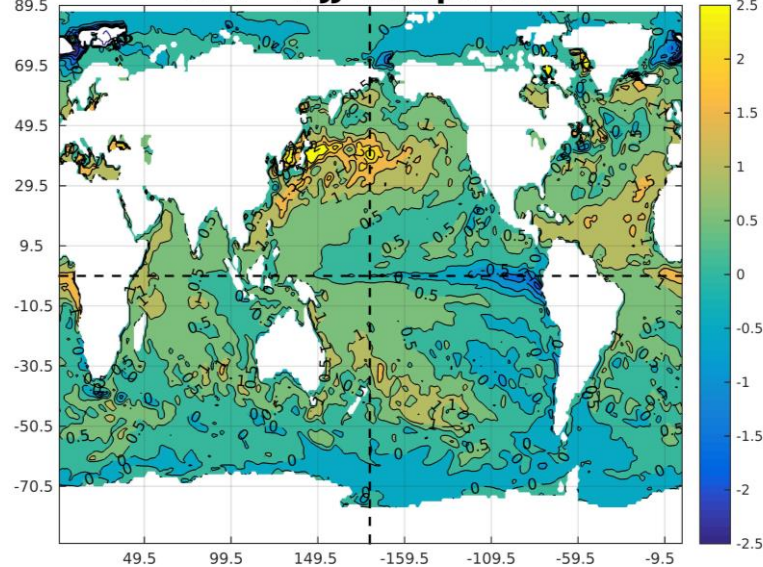
SST MJJ IC:Apr2024
