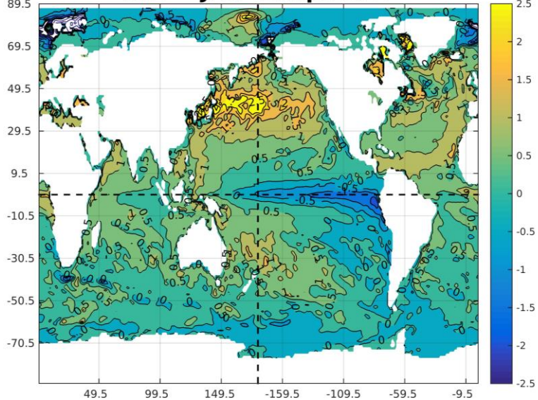
SST JAS IC:Apr2024
