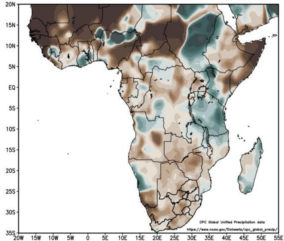
Rainfall (% of normal): January–February–March 2024 January–February–March long-term mean: 1981–2010
