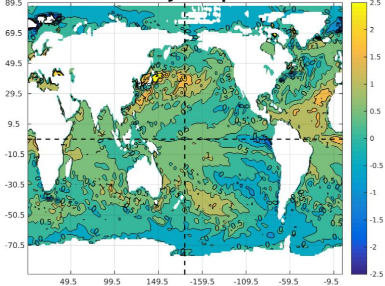
SST AMJ IC:Apr2024
