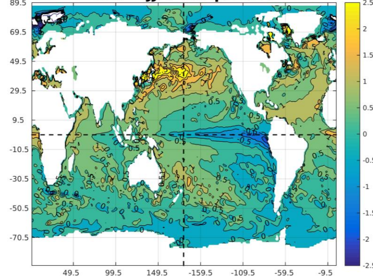
SST JJA IC:Apr2024
