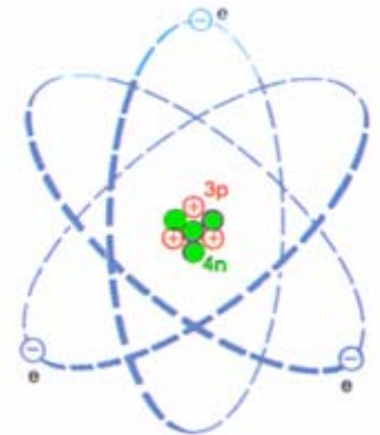
Lithium Atom
