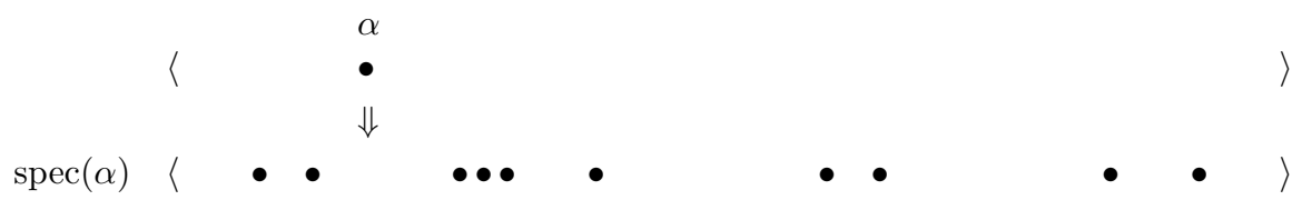
Figure A. Each real number \alpha determines \text{spec}(\alpha) , a countably infinite subset of the reals.
